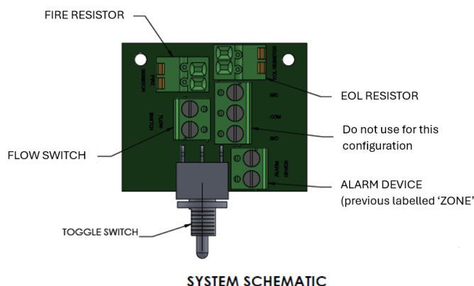
SYSTEM SCHEMATIC
