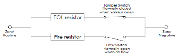
SYSTEM SCHEMATIC
