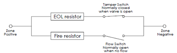
SYSTEM SCHEMATIC
