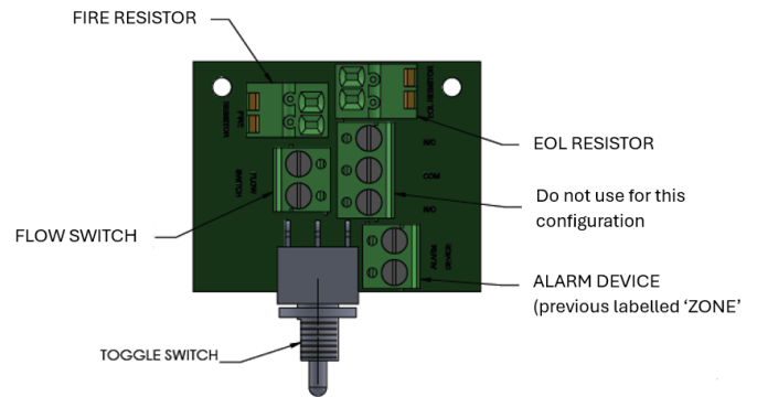
SYSTEM SCHEMATIC
