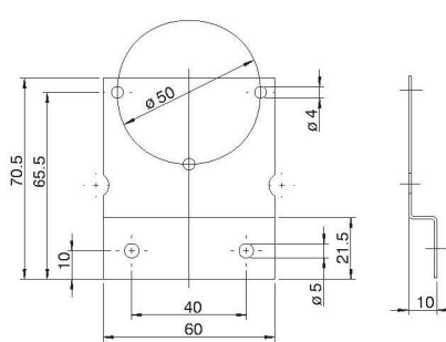
Mounting bracket 6402
