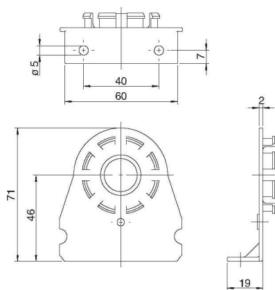
Mounting bracket 6482
